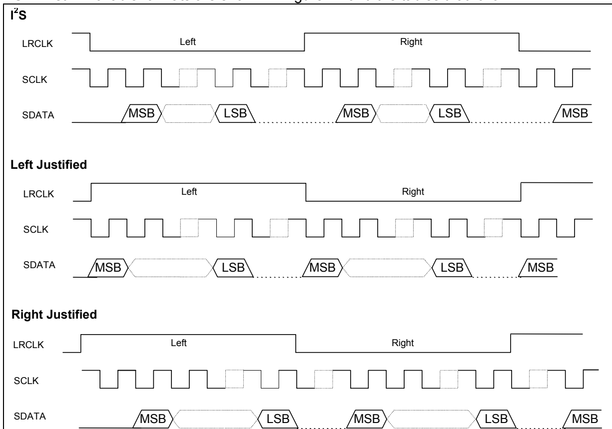
Figure 24 - Serial Audio Input and Output Formats
