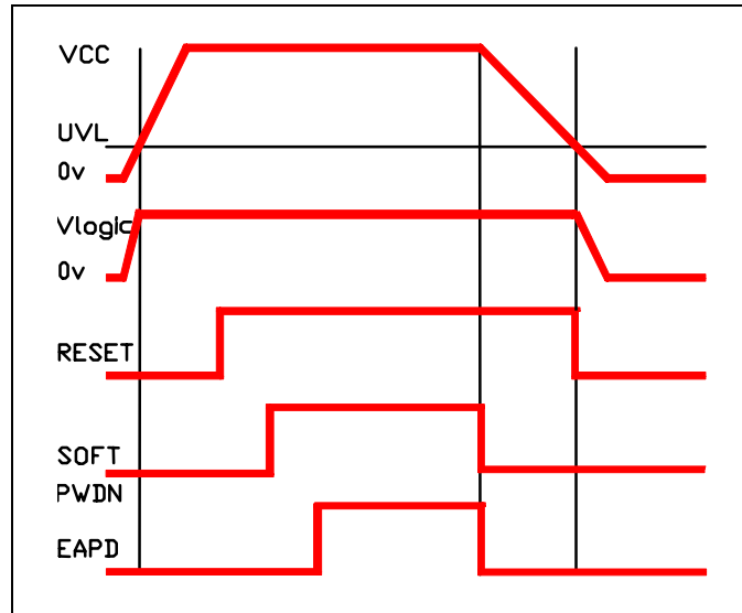
Figure 32 – Recommended Power-Up & Power-Down Sequence
