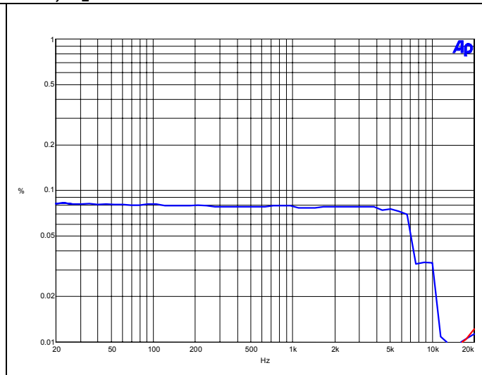
Figure 15 - THD vs. Frequency, 1W
