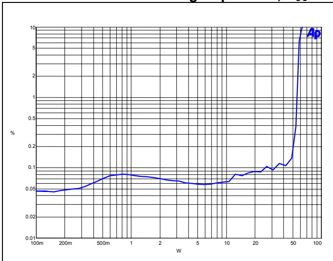
Figure 14 - THD vs. Power, 1kHz
