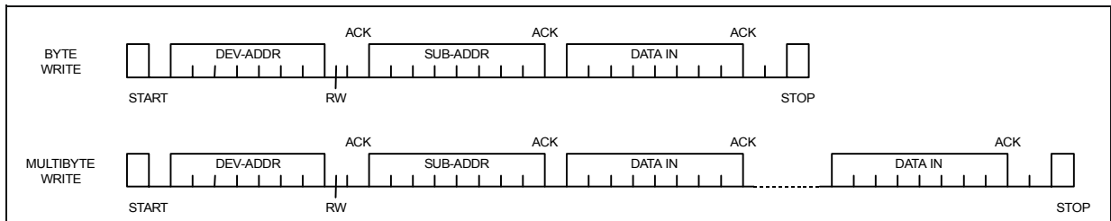
Figure 22 - I 2 C Write Procedure
