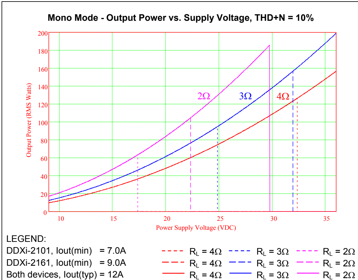
Figure 30 - Mono Bridge Output, DDX Mode Only, Power vs. Supply [Note 8]
