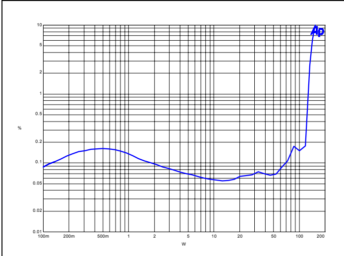
Figure 16 - THD vs. Power, 1kHz
