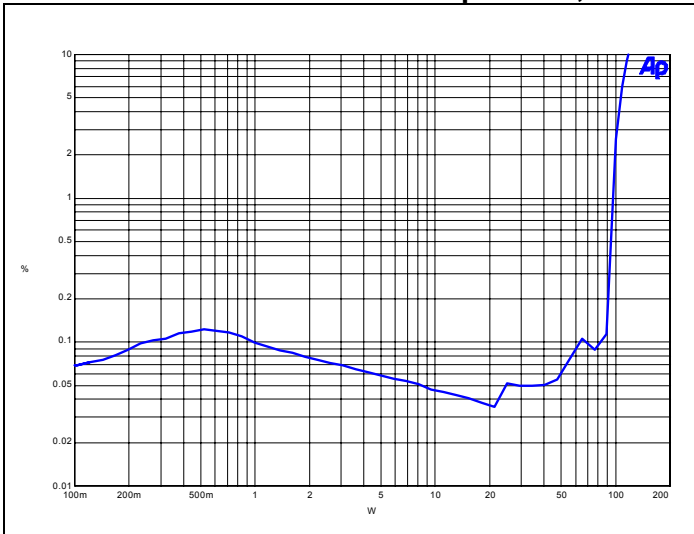
Figure 18 - THD vs. Power, 1kHz
