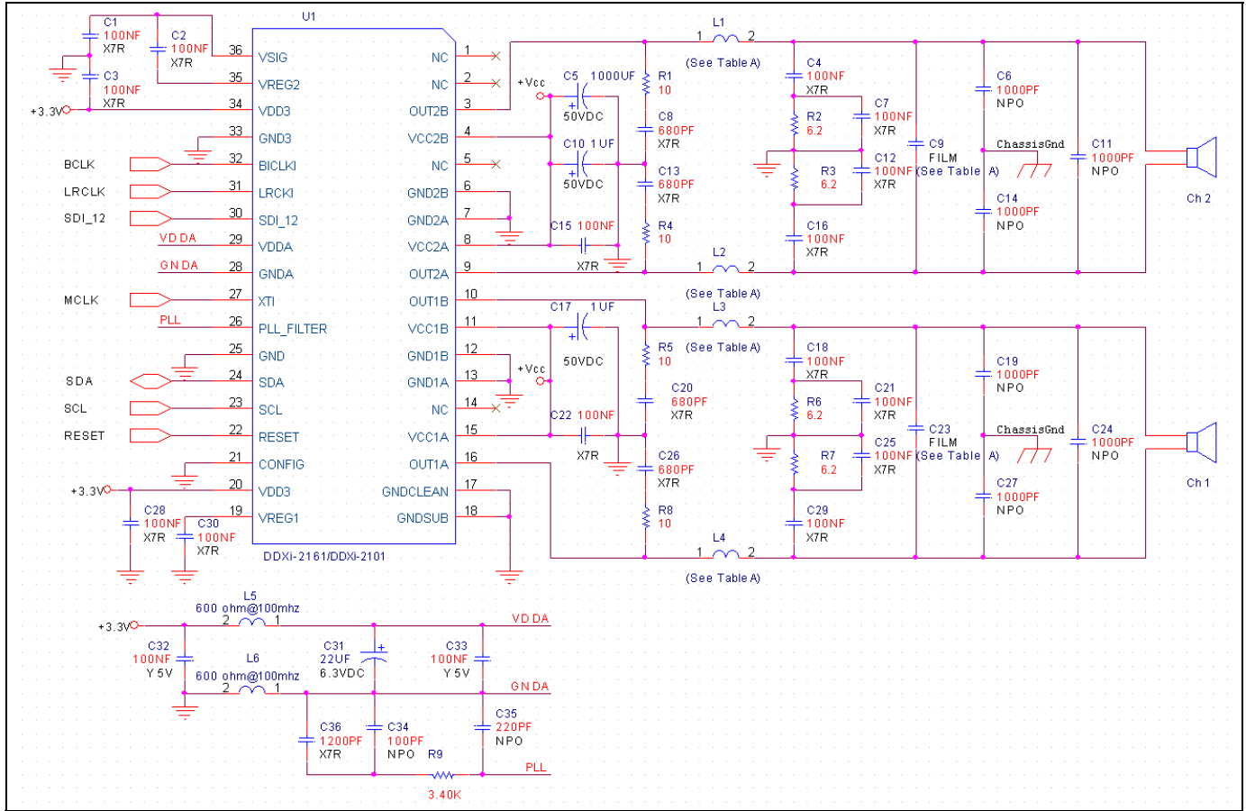
Figure 34 - Schematic Diagram for 2-channel (Full-bridge) Power.
