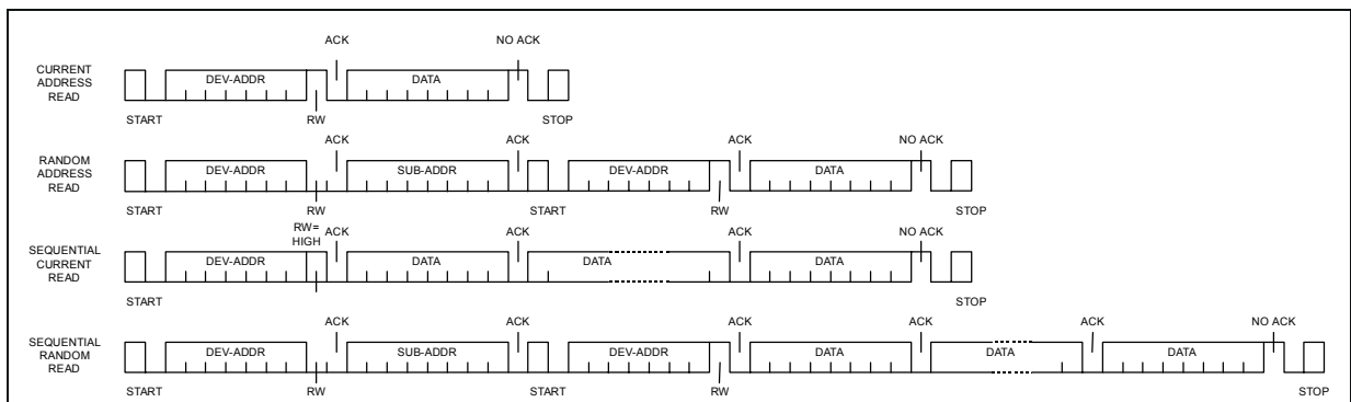
Figure 23 - I 2 C Read Procedure
