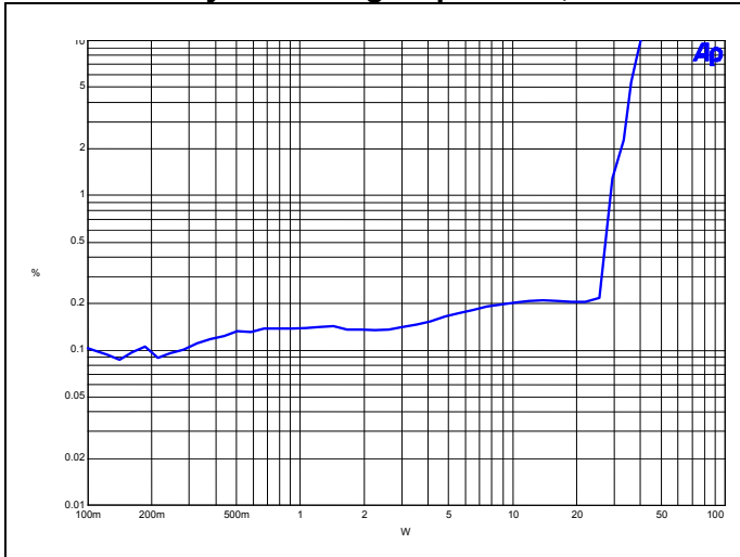
Figure 20 - THD vs. Power, 1kHz
