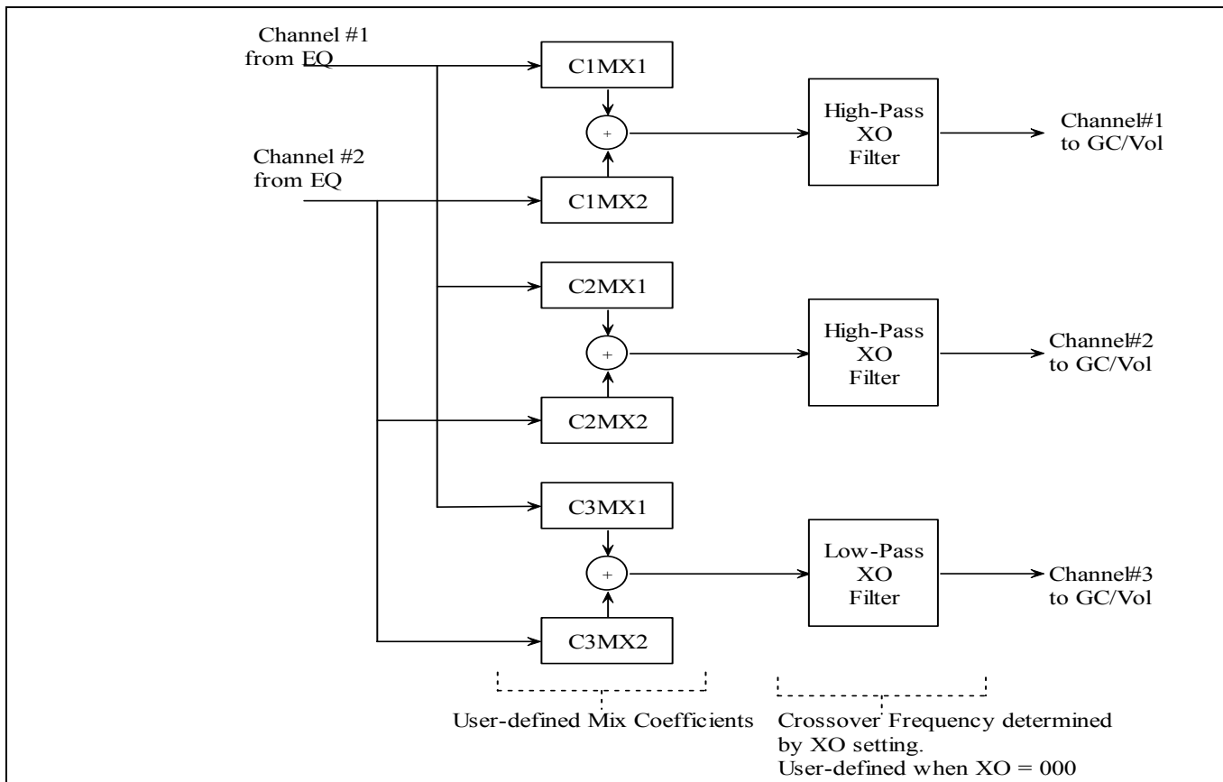
Figure 28 - Mix/Bass Management Block Diagram
