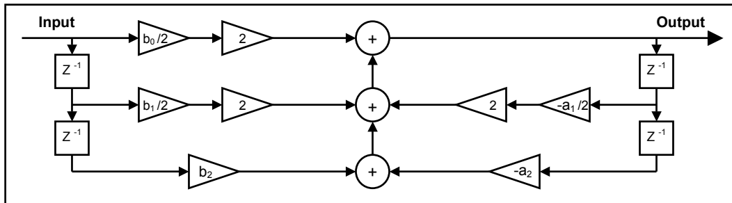
Figure 27 - Biquad Filter Structure
