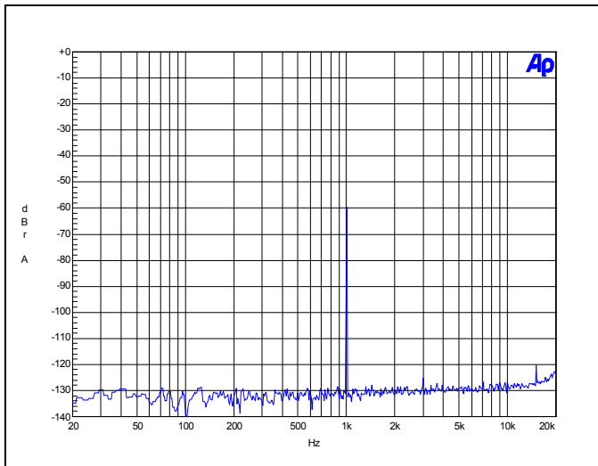
Figure 10 - FFT -60dB, 1kHz Output
