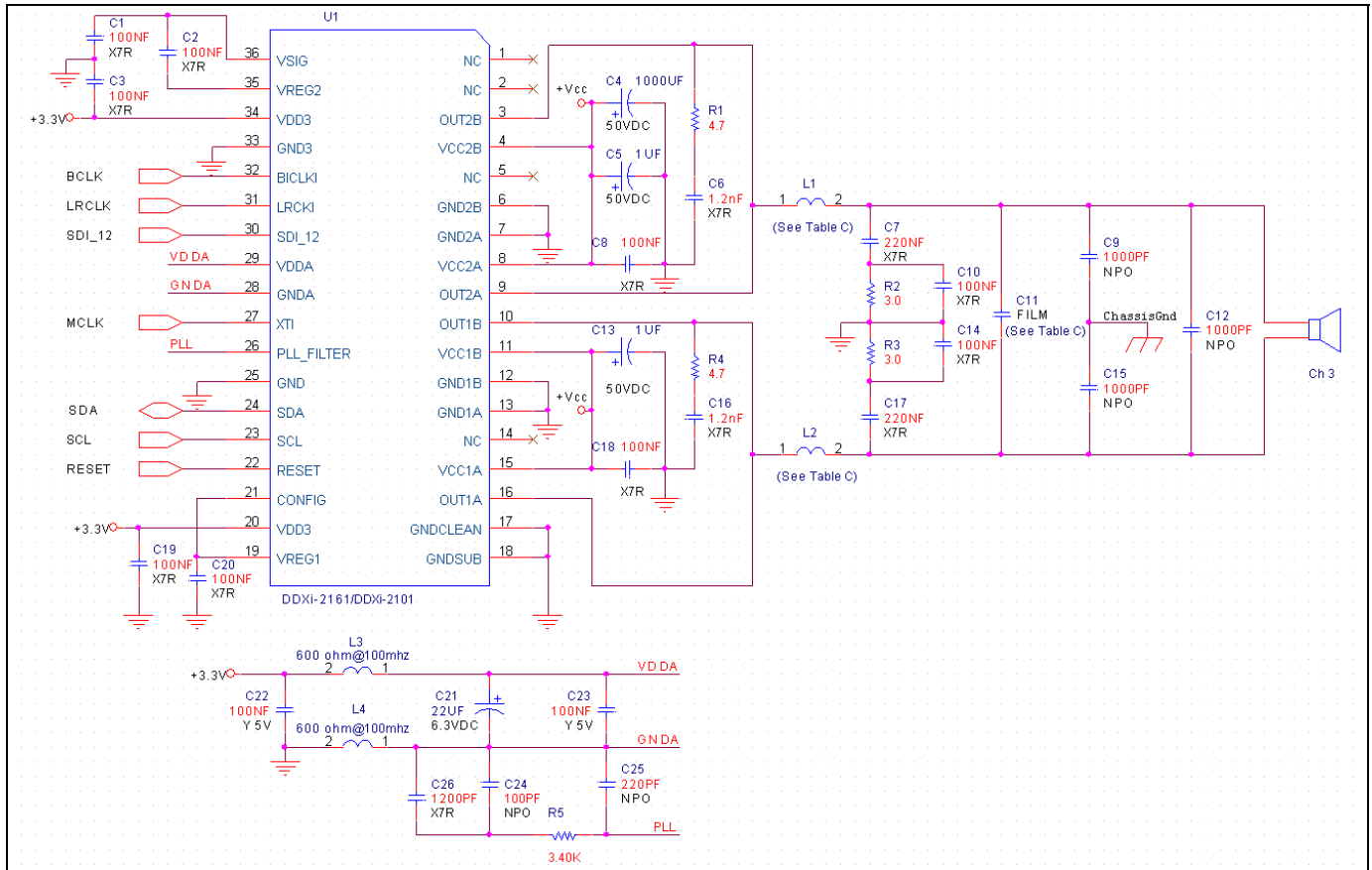
Figure 35 - Schematic Diagram for 1-channel Mono-Parallel Power.
