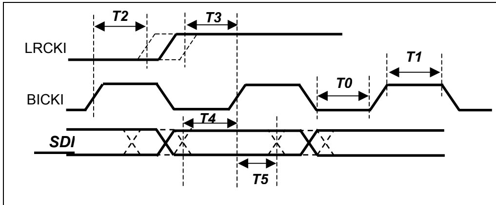
Figure 25 - Serial Input Data Timing Characteristics
