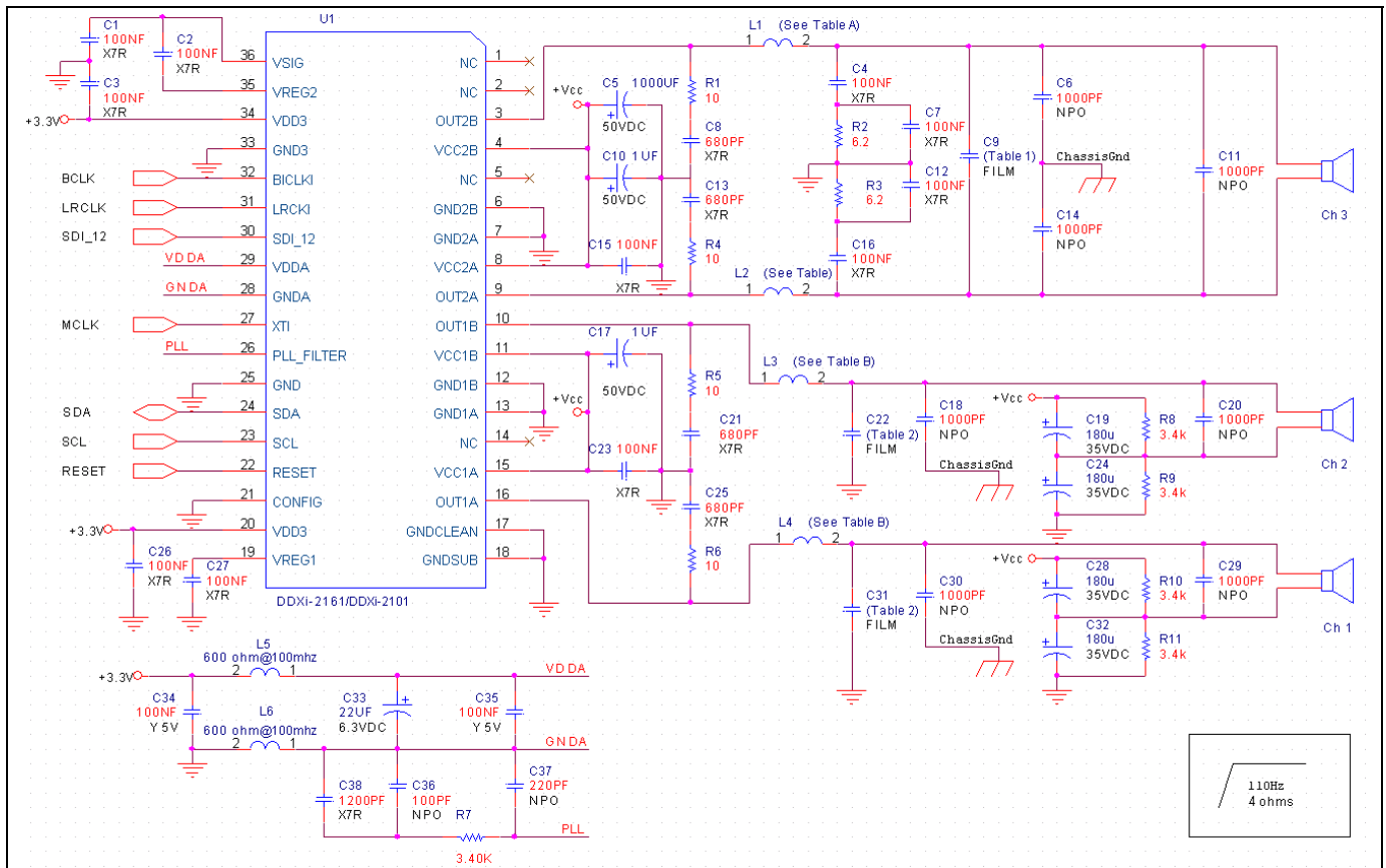
Figure 33 - Schematic Diagram for 2(Half-bridge).1(Full-bridge)-channel On-board Power.
