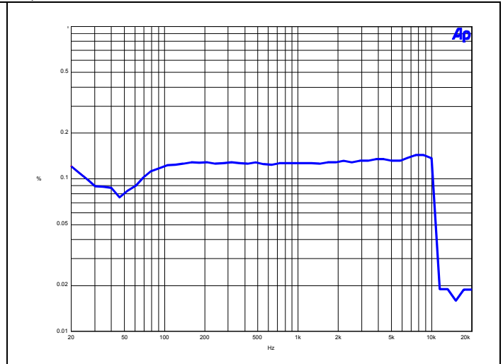
Figure 21 - THD vs. Frequency, 1W
