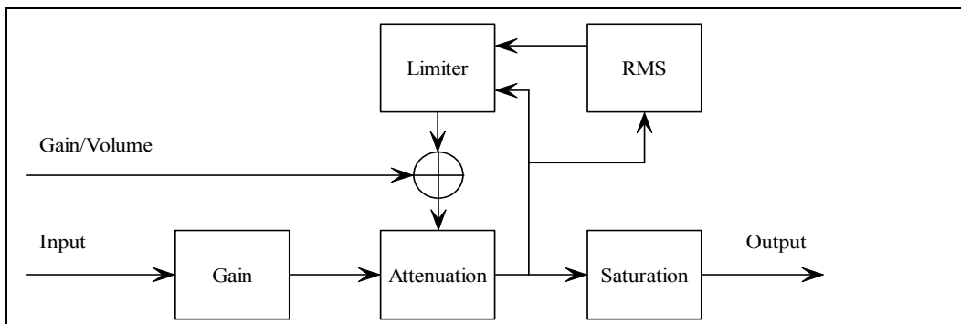
Figure 26 - Basic Limiter and Volume Flow Diagram.
