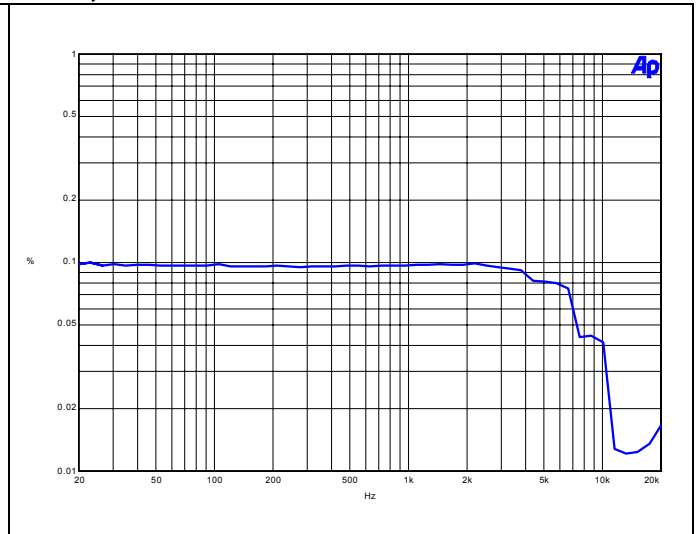
Figure 19 - THD vs. Frequency, 1W
