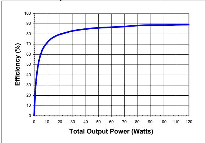
Figure 8 - Typical Efficiency
