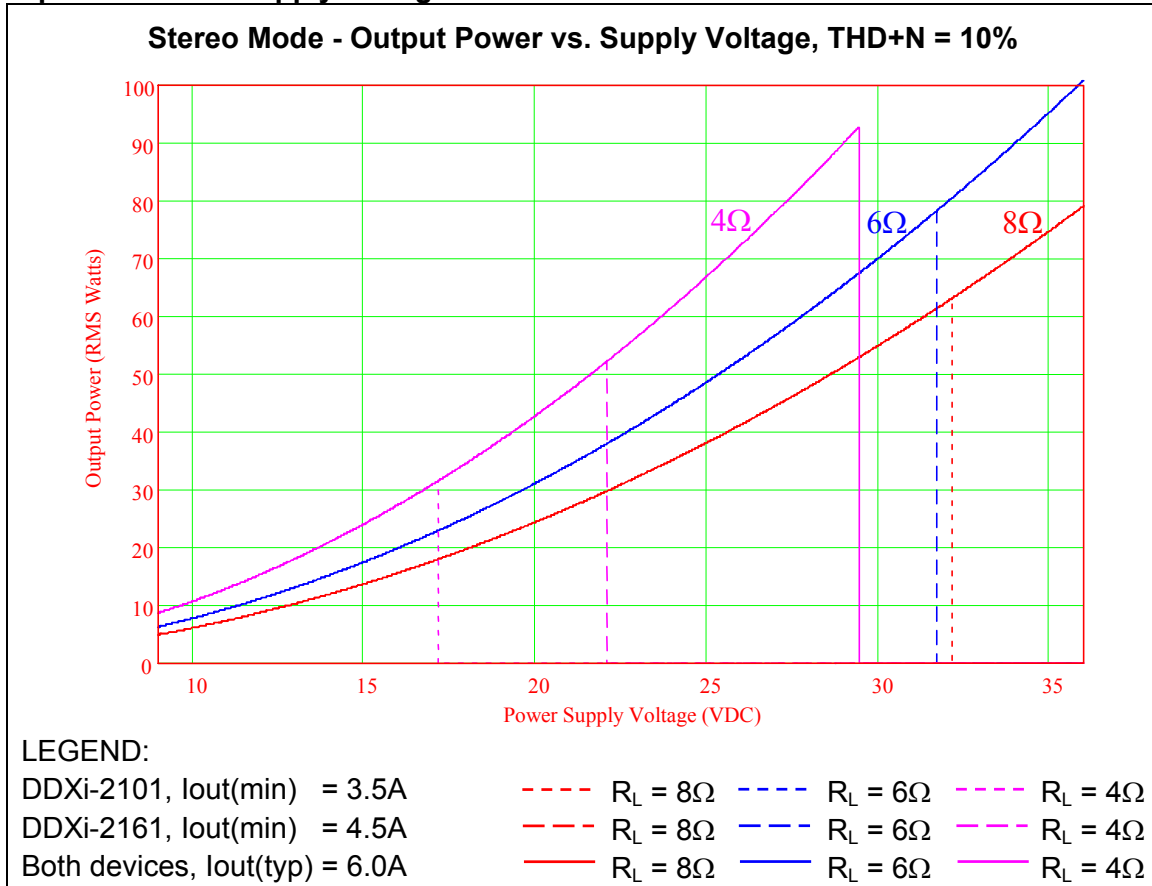
Figure 29 - Output Power vs. Supply Voltage for Stereo Bridge
