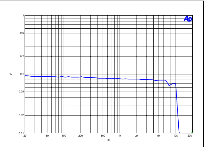
Figure 13 - THD vs. Frequency, 1W
