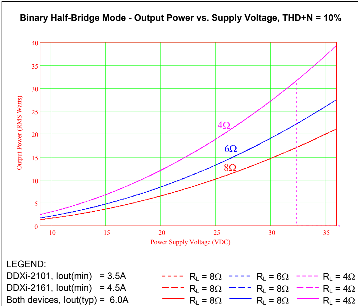
Figure 31 - Half-Bridge Binary Mode Output Power vs Supply [Note 9] [Note 10]
